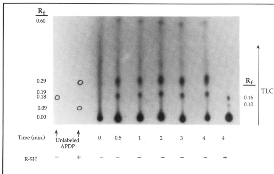
FIGURE 1: Iodination APDP by high specific activity [ ^{125}\text{I} ]NaI. Samples of the iodination reaction mixture were removed at the indicated times and analyzed by thin-layer chromatography and autoradiography.
