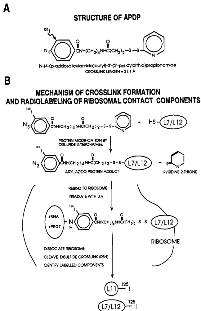
FIGURE 2: The structure of APDP and its mechanism of cross-linking. (A) The structure of the sulfhydryl-specific, heterobifunctional, photoactivatable cross-linking reagent APDP. Radiolabeling with ^{125}\text{I} is indicated by an arrow. The maximum length of the cross-bridge is 21.1 Å. (B) Scheme for APDP mediated cross-link formation and radiolabeling of binding site components.
