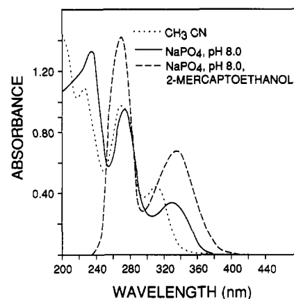
FIGURE 3: Absorbance spectrum of APDP and effect of reduction. APDP dissolved in acetonitrile was diluted into aqueous buffer with or without 2-mercaptoethanol, as indicated. (---) 50 \mu\text{M} APDP in \text{CH}_3\text{CN} ; (—) 50 \mu\text{M} APDP in 50 mM \text{NaPO}_4 , pH 8.0; (---) 50 \mu\text{M} APDP in 50 mM \text{NaPO}_4 , pH 8.0, with 50 mM 2-mercaptoethanol.
